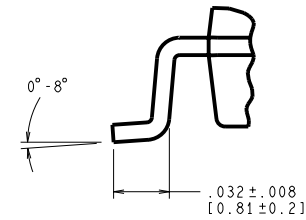
DETAIL A TYPICAL, SCALE: 20X
